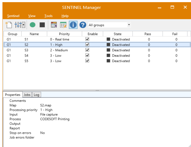
Figure 7: Sentinel Manager window
