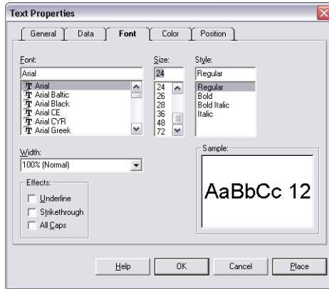
Figure 7 Font Tab
