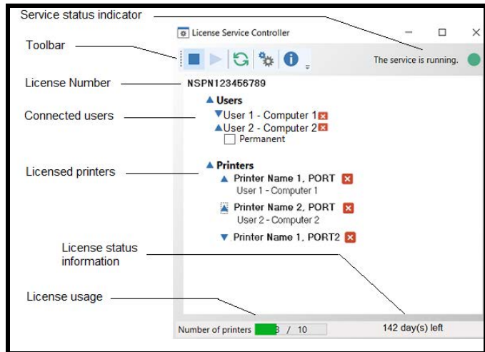
그림 5: Main Service Control window for licenses limited by printers
