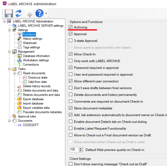
Figure 3 Version Control
