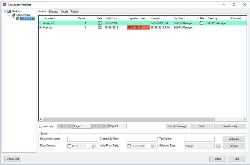
Figure 12 Versions window
