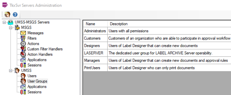
Figure 8 Sample of user groups in UMSS ADMINISTRATION
