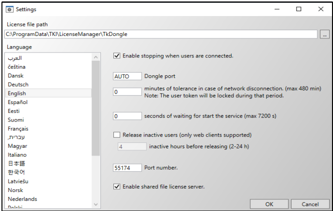
Figure 5: Settings window
