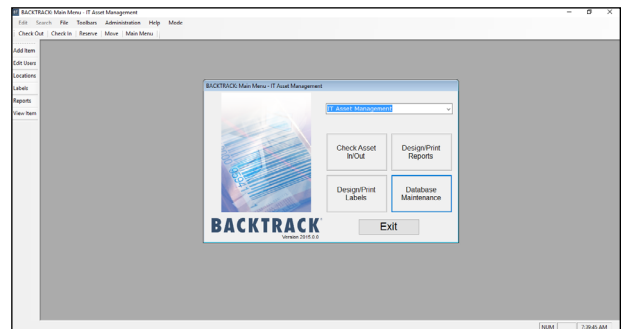
Main Menu
