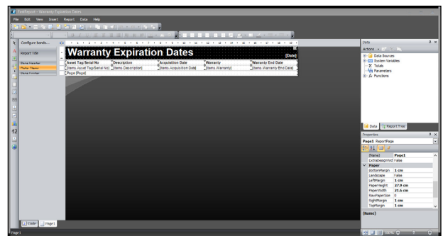
Report Designer
